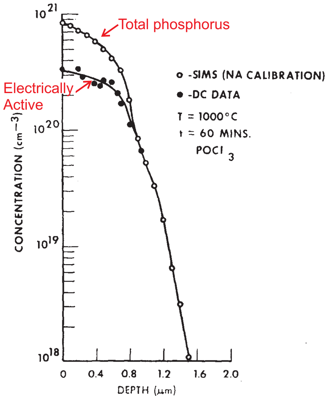
Figure 1. Electrically active and inactive phosphorus for a high surface concentration. Used with permission of the Electrochemical Society. After R. B. Fair and J. C. C. Tsai, "A quantitative model for diffusion of phosphorus in silicon and the emitter dip effect", Journal of the Electrochemical Society , 124(7):1107-1118, 1977.
